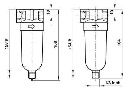
Dreno manual
